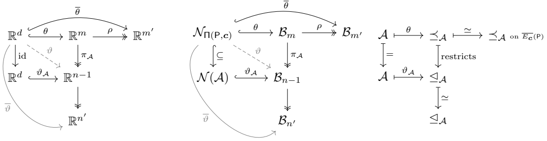
Figure 51: (Middle) The linear maps and projections that embeds the normal fan of \Pi(P, c) into braid fans of different dimensions. (Left) The real vector spaces these maps have for domains. (Right) Utter and adapted pre-orders associated to the multi-arborescence, and their restrictions.
