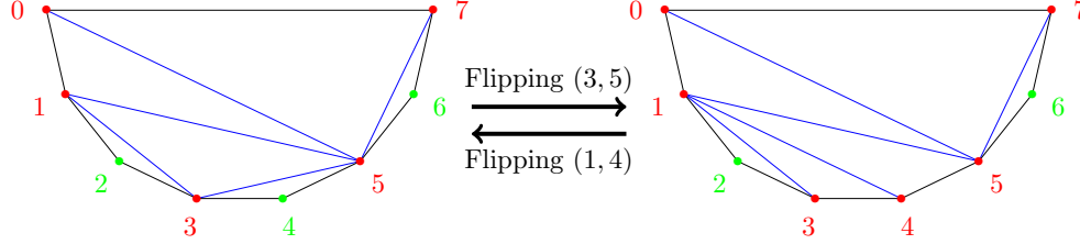
Figure 70: (Left) The triangulation T = ((0, 5, 7), (0, 1, 5), (1, 3, 5), (1, 2, 3), (3, 4, 5), (5, 6, 7)) . Its 8 exterior edges are in black, while its 5 interior ones are in blue . It has 2 positive quadrangles and 3 negative ones: Q^+(T) = ((0, 1, 5, 7), (1, 2, 3, 5)) and Q^-(T) = ((0, 1, 3, 5), (0, 5, 6, 7), (1, 3, 4, 5)) . Its immediate vertices are in green: \mathbb{L}(T) = \{2, 4, 6\} . Flipping the edge (3, 5) gives the triangulation T' on the Right. The new quadrangles are Q^+(T') = ((0, 1, 5, 7), (1, 3, 4, 5), (1, 2, 3, 4)) and Q^-(T') = ((0, 5, 6, 7), (0, 1, 4, 5)) , and new immediate vertices are \mathbb{L}(T') = \{2, 6\} . Flipping the edge (1, 4) in T' gives back T .
