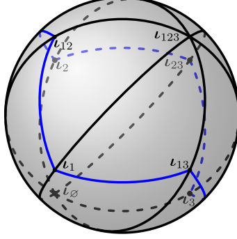
Figure 11: The fan \widehat{\mathcal{B}}_{123} intersected with the unit sphere. (For brevity, here and in the labels we write 123 to denote the set \{1, 2, 3\} , and so on.) The braid fan \mathcal{B}_{123} is the Cartesian product of a regular hexagonal fan with a line. To obtain \widehat{\mathcal{B}}_{123} , each maximal cell is divided into two simplicial cells, one containing \iota_{\emptyset} and one containing \iota_{123} .
