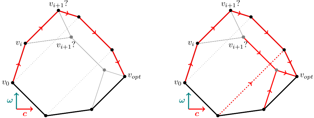
Figure 25: (Left) In red, the coherent monotone path associated to the parameter \omega for the linear problem (P, c) . (Right) In red, the coherent arborescence associated to the same parameter. In both figures, to each vertex, the pivot rule associates the one of its neighbors that maximizes the slope in the plane (c, \omega) .
