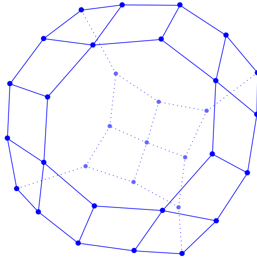
Figure 60: The monotone path polytope M(5,2) of the hypersimplex \Delta(5,2) . This hypersimplex is linearly equivalent to \Delta(5,3) . As \Delta(5,2) has 5 facets linearly equivalent to \Delta(4,2) , its monotone path polytope M(5,2) has 5 facets which are isomorphic to M(4,2) i.e. octagons.
