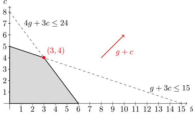
Figure 8: Feasibility domain, objective function and optimal vertex of the toy example.
