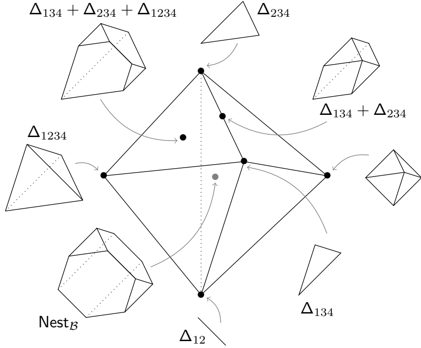
Figure 23: A 3-dimensional affine section of the deformation cone \mathbb{DC}(\mathcal{F}(\mathcal{B})) for the building set of Example 2.65 and Figure 22. The deformations of \text{Nest}_{\mathcal{B}} corresponding to some of the points of \mathbb{DC}(\mathcal{F}(\mathcal{B})) are depicted. Especially, all points in the interior correspond to polytopes normally equivalent to \text{Nest}_{\mathcal{B}} , while the rightmost polytope is not a simplex. See also Figure 12 for the case of the complete graph on 3 vertices.
