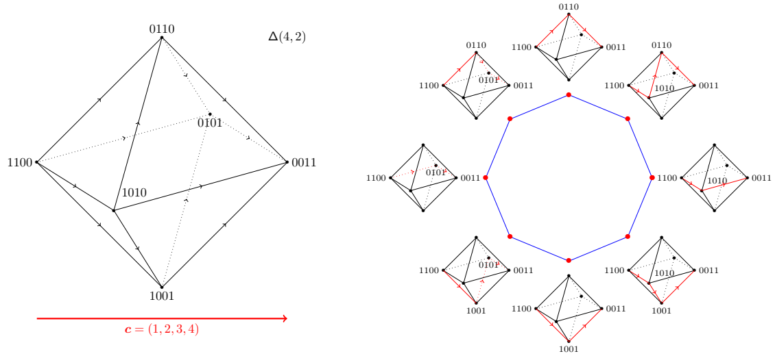
Figure 59: (Left) The (4,2) -hypersimplex lives in the hyperplane \{x ; \sum_{i=1}^4 x_i = 2\} inside \mathbb{R}^4 . (Right) The monotone path polytope M(4,2) is an octagon, each vertex of which is labelled by the corresponding monotone path (drawn on \Delta(4,2) ).
