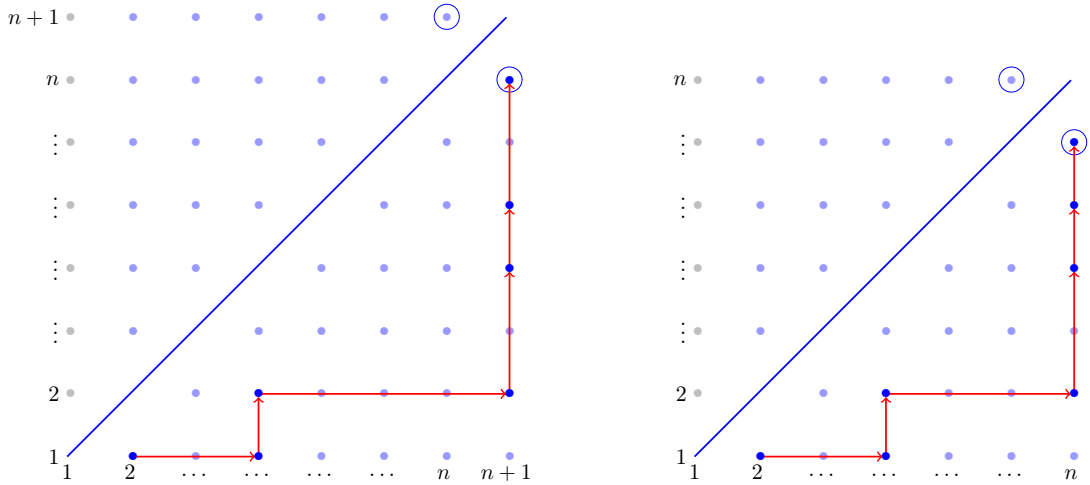
Figure 65: The restriction of \mathcal{L} to \mathcal{L}' restrict its enhanced steps from \mathcal{S}(\mathcal{L}) = (2 \xrightarrow{1} 4, 1 \xrightarrow{4} 2, 4 \xrightarrow{2} n+1, 2 \xrightarrow{n+1} 4, 4 \xrightarrow{n+1} 5, 5 \xrightarrow{n+1} n) to \mathcal{S}(\mathcal{L}') = (2 \xrightarrow{1} 4, 1 \xrightarrow{4} 2, 4 \xrightarrow{2} n, 2 \xrightarrow{n} 4, 4 \xrightarrow{n} 5, 5 \xrightarrow{n} n-1) .
