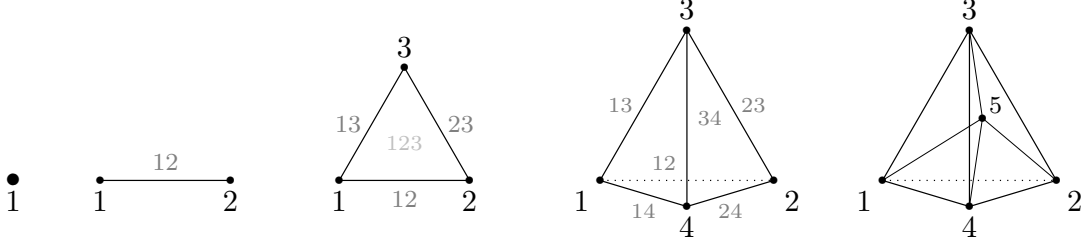
Figure 2: The standard simplices for dimension d = 0, 1, 2, 3 and 4 (from Left to Right). Each face is labelled by the corresponding subset of [d] . The 4-dimensional standard simplex (Right) is depicted thanks to its Schlegel projection.
