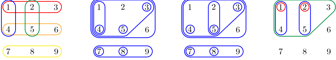
Figure 18: The elementary blocks of a building set \mathcal{B}_0 (Left), two adjacent maximal \mathcal{B}_0 -nested sets (Middle), and the corresponding frame (Right).
