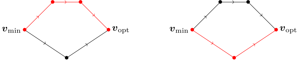
Figure 9: The two possible monotone paths starting at the minimal vertex for a 2-dimensional polytope (the objective function is from left to right).
